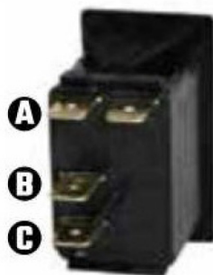
FIG 4 & FIG 5 - Connect the Black, White, and Blue wires to the switch. Connect the ring terminals of the harness to the under hood busbar
