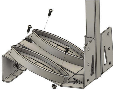
FIG 3 - Mount Gun Butts to the Attachment Plate
