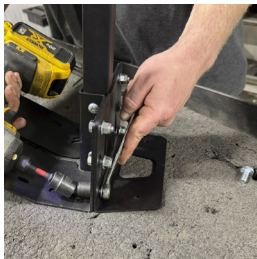
FIG 5 - Mount the Floor Mount - Gusset Plate to the Base
