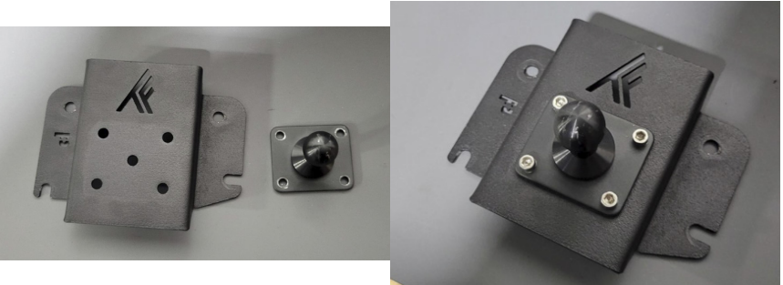
FIG 3 & 4 - Mount ball mount to mount bracket using 9/64" Allen and 11/32" Wrench
