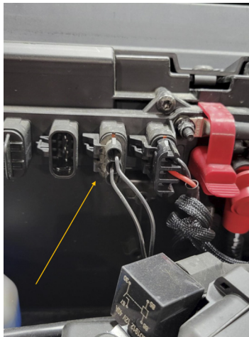
FIG 8 - Connect wiring harness to the pulse bar
