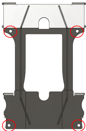
FIG 4 & FIG 5 - Drill holes through frame using the Base as a template
