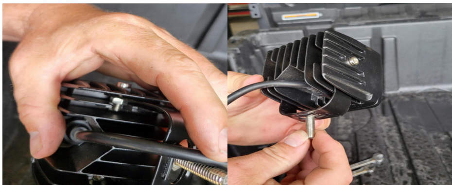
FIG 20 & FIG 21 - Fasten Cube Light to Mount Bracket
