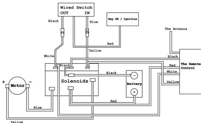
FIG 14 - Winch Wiring Diagram
