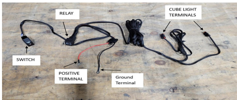
FIG 24 - Wiring Harness Breakdown of Plugs and Terminals
