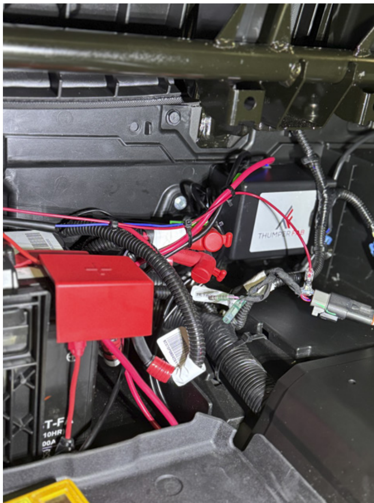
FIG 17 - Mount location for winch contactor box (HD11 ONLY)
