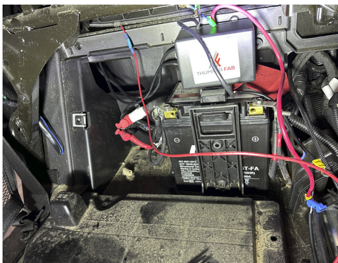
FIG 16 - Mount Winch Control Box
