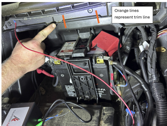
FIG 15 - Grind down plastic lip for Winch Control Box
