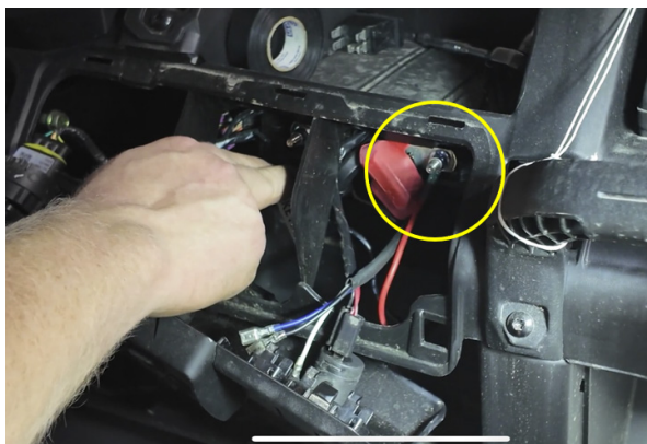
FIG 19 - Connect Winch Wires
