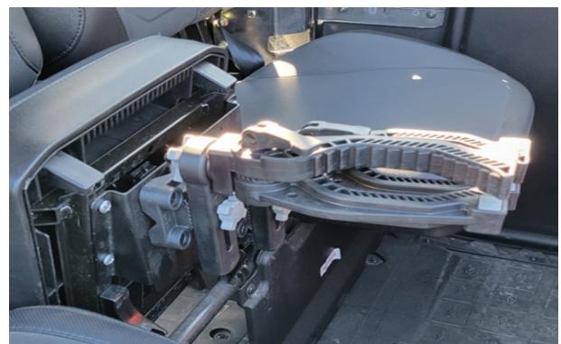
FIG 3 & FIG 4 - Using #3 Phillips Bit and Drill attach Plate to underside of Seat
