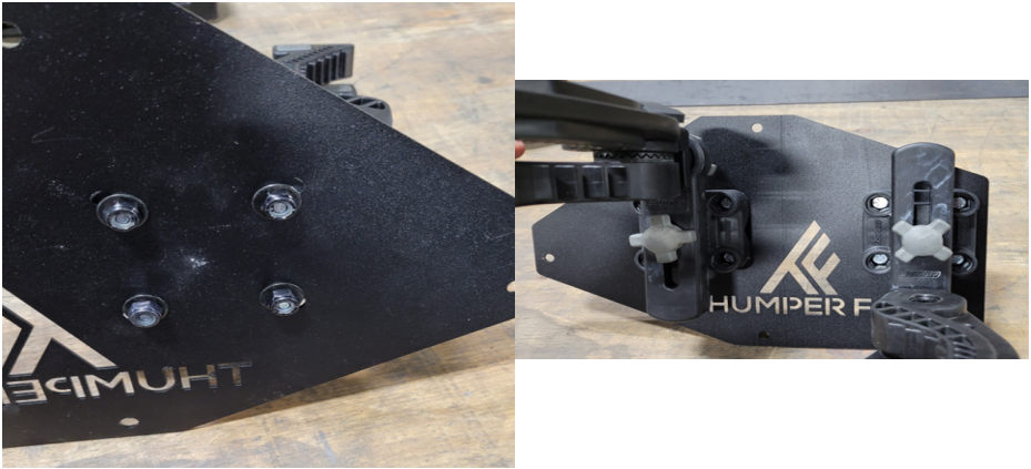
FIG 1 & FIG 2 - Mount Gun Calmps to Mount Plate using a 7/16" Socket
